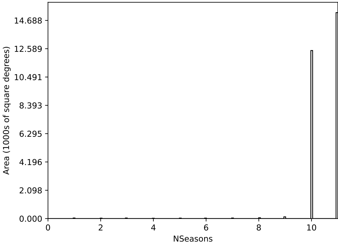
ddf_acor_sf20_lsf30_lsr10_v3.4_10yrs All sky all bands: NSeasons
