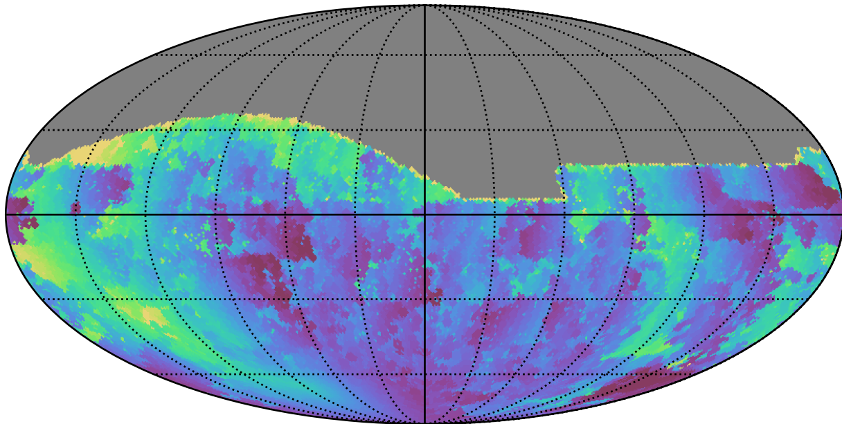
ddf_acor_sf20_lsf30_lsr10_v3.4_10yrs All sky g band: Min solarElong
