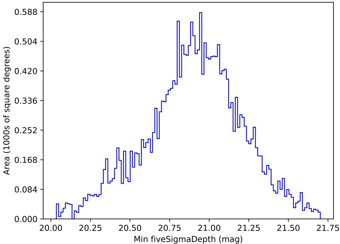
ddf_acor_sf20_lsf30_lsr10_v3.4_10yrs All sky y band: Min fiveSigmaDepth
