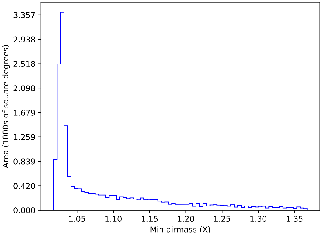
ddf_acor_sf20_lsf30_lsr10_v3.4_10yrs WFD i band: Min airmass
