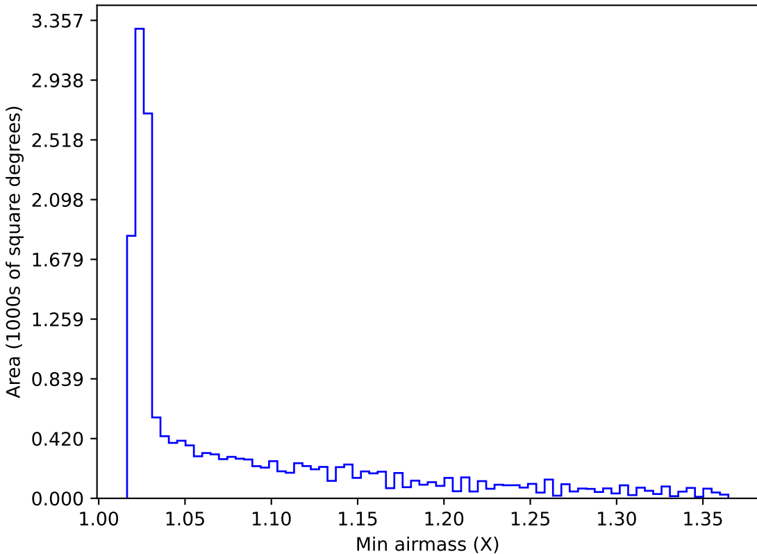
ddf_acor_sf20_lsf30_lsr10_v3.4_10yrs WFD all bands: Min airmass
