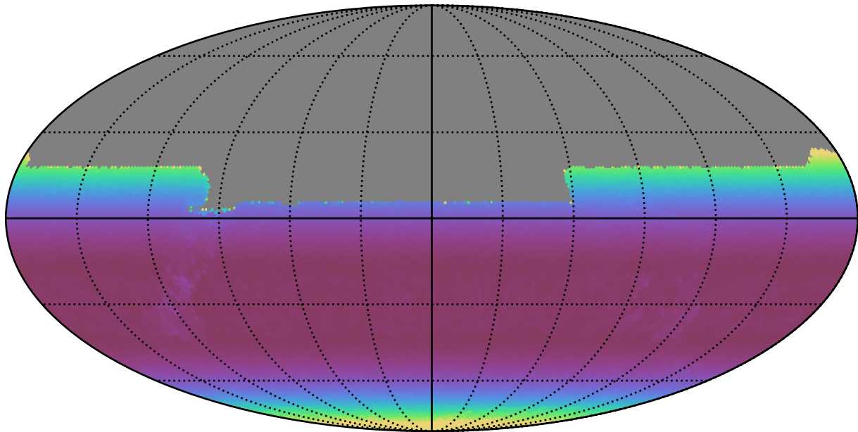
ddf_acor_sf20_lsf30_lsr10_v3.4_10yrs All sky y band: Min airmass
