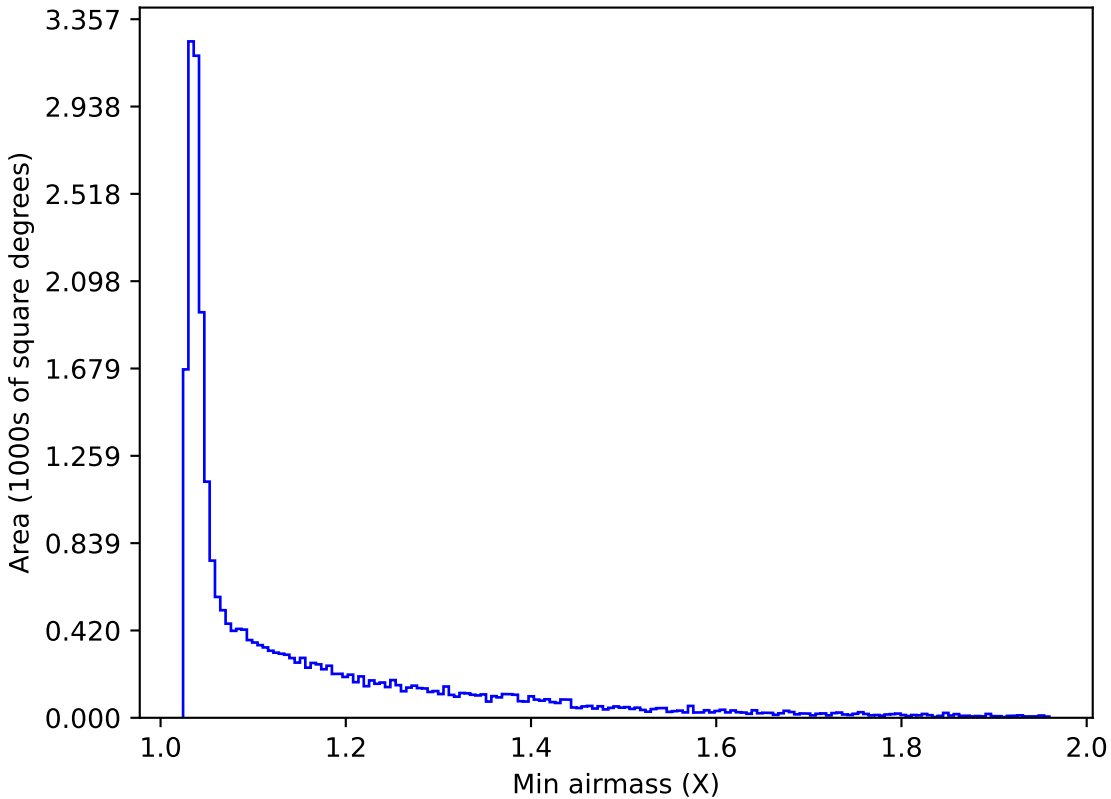
ddf_acor_sf20_lsf30_lsr10_v3.4_10yrs All sky g band: Min airmass
