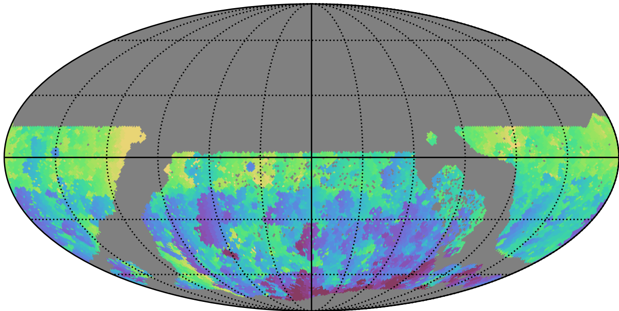
ddf_acor_sf20_lsf30_lsr10_v3.4_10yrs WFD u band: Min HA
