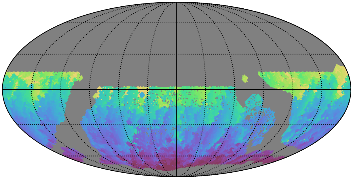
ddf_acor_sf20_lsf30_lsr10_v3.4_10yrs WFD g band: Min HA
