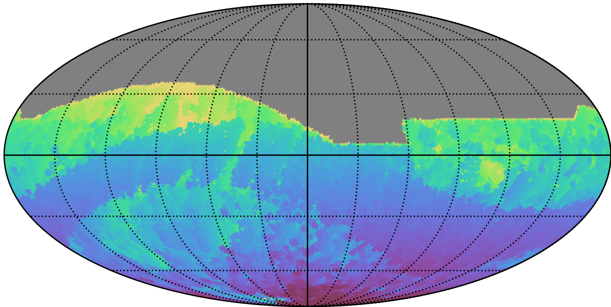
ddf_acor_sf20_lsf30_lsr10_v3.4_10yrs All sky r band: Min HA
