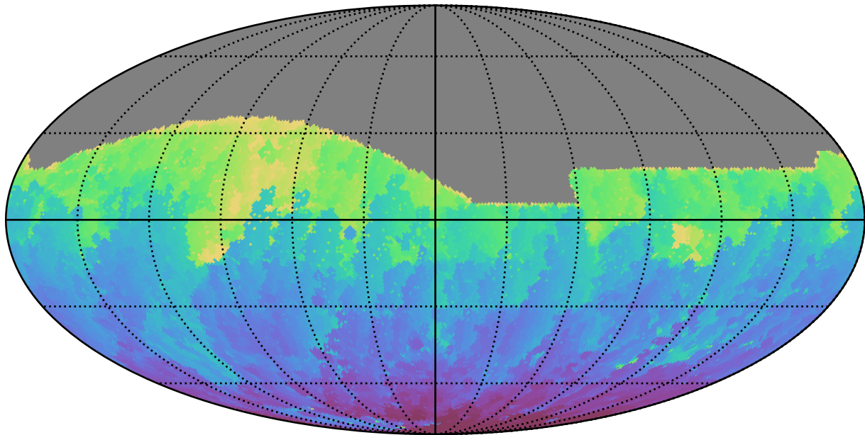
ddf_acor_sf20_lsf30_lsr10_v3.4_10yrs All sky g band: Min HA
