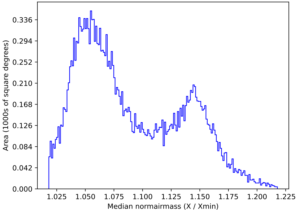
ddf_acor_sf20_ls30_lsr10_v3.4_10yrs All sky y band: Median normairmass
