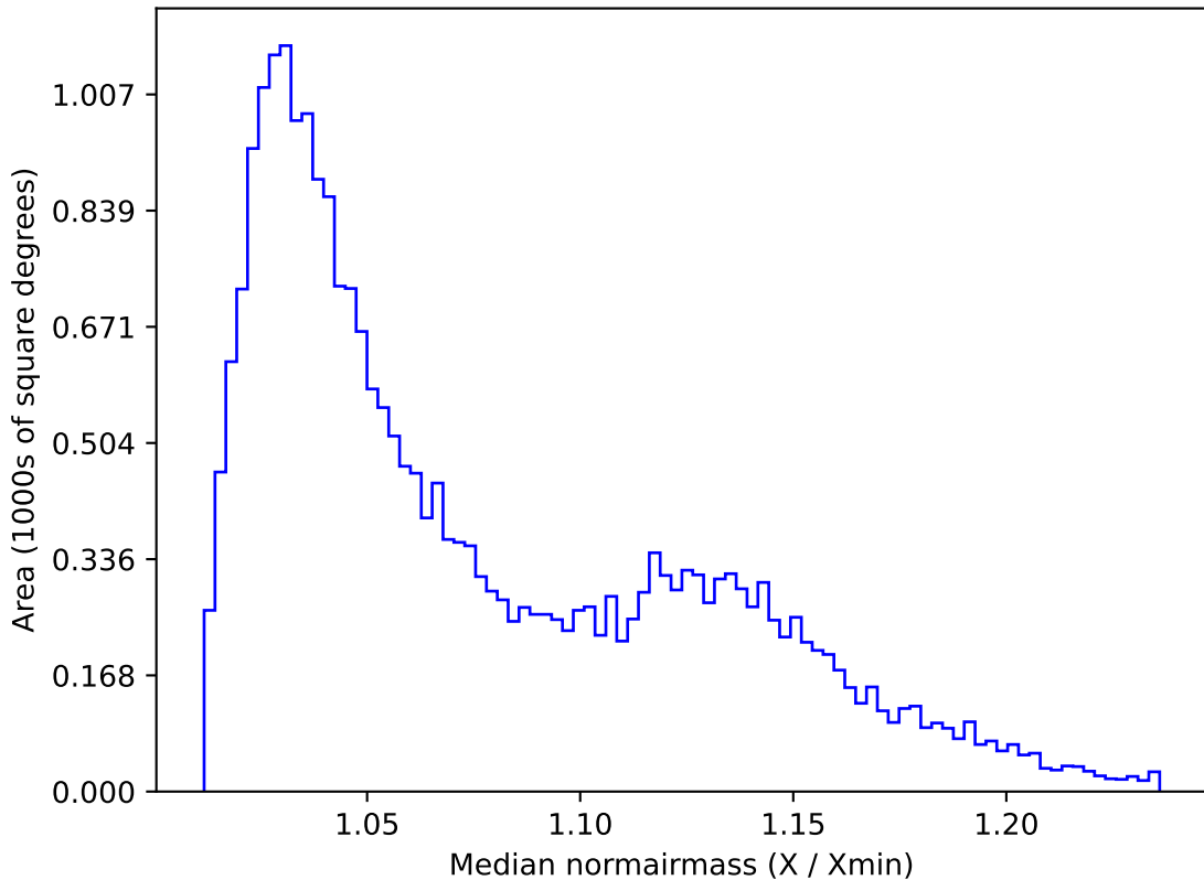
ddf_acor_sf20_lsf30_lsr10_v3.4_10yrs All sky g band: Median normairmass
