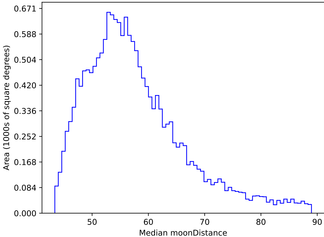
ddf_acor_sf20_lsf30_lsr10_v3.4_10yrs WFD y band: Median moonDistance
