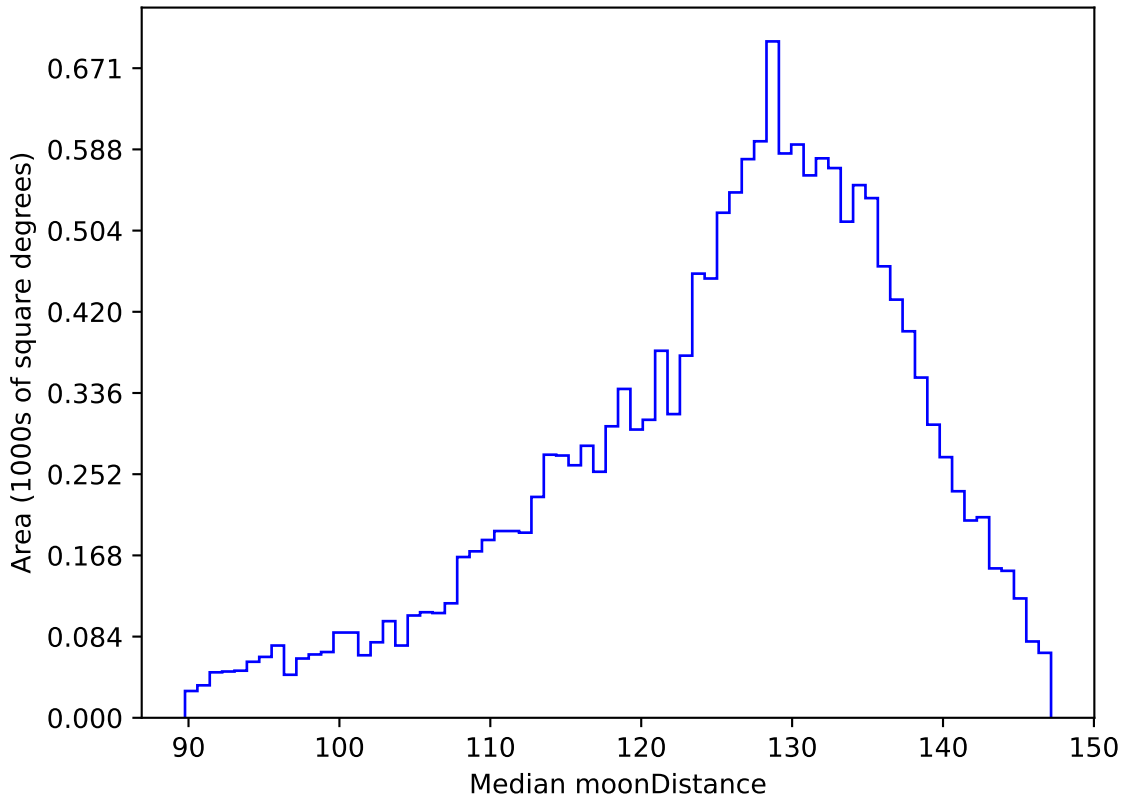
ddf_acor_sf20_ls30_lsr10_v3.4_10yrs WFD u band: Median moonDistance
