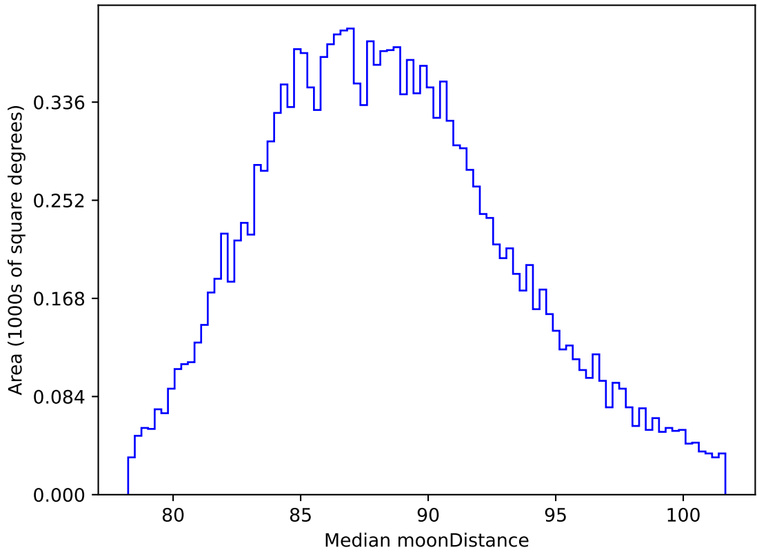
ddf_acor_sf20_lsf30_lsr10_v3.4_10yrs WFD all bands: Median moonDistance
