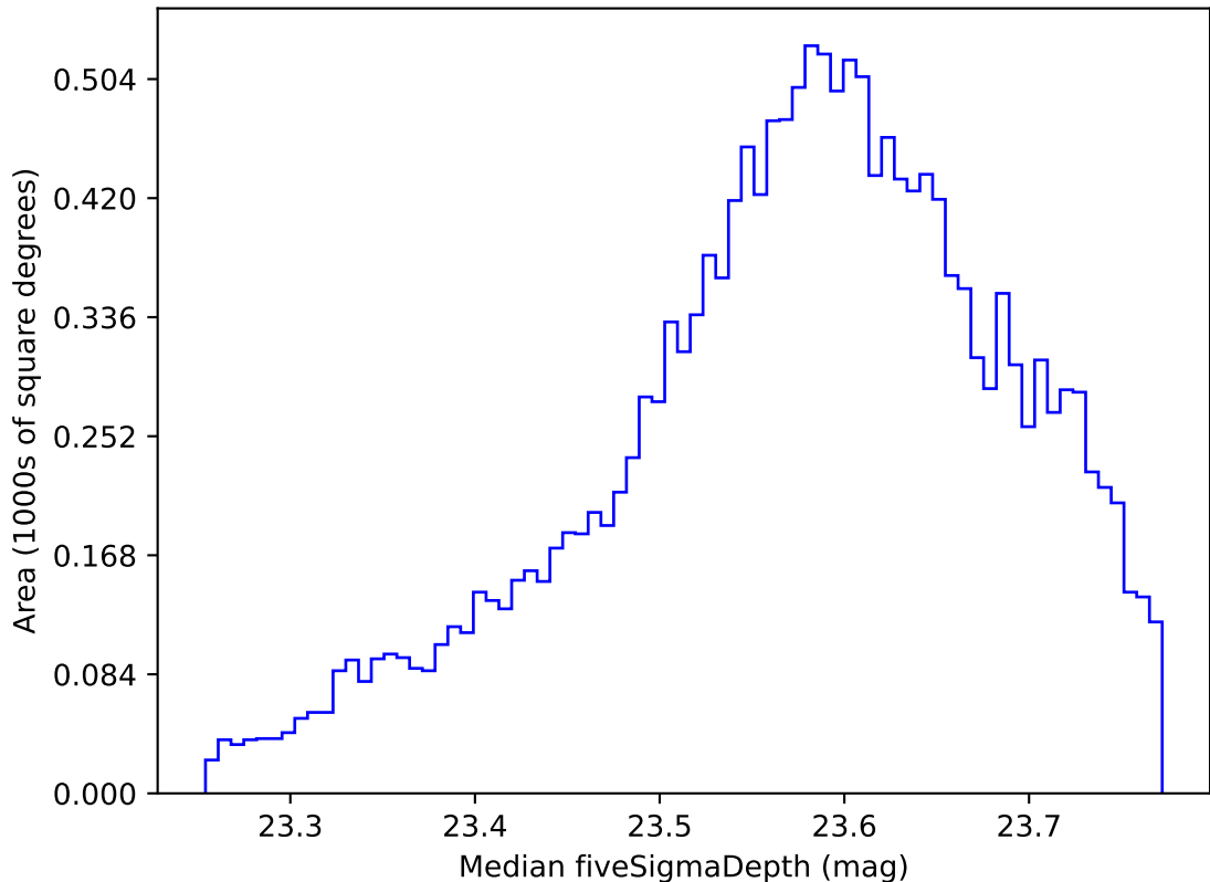
ddf_acor_sf20_lsf30_lsr10_v3.4_10yrs WFD i band: Median fiveSigmaDepth
