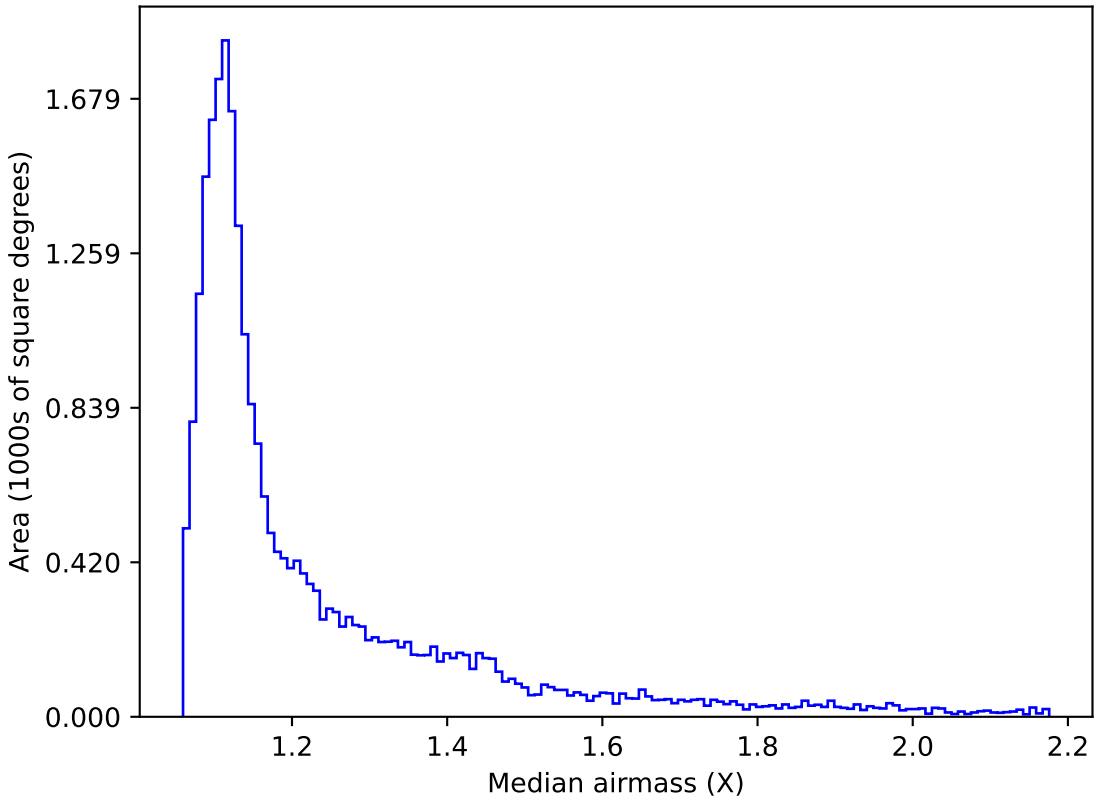
ddf_acor_sf20_lsf30_lsr10_v3.4_10yrs Yr 1 i band: Median airmass
