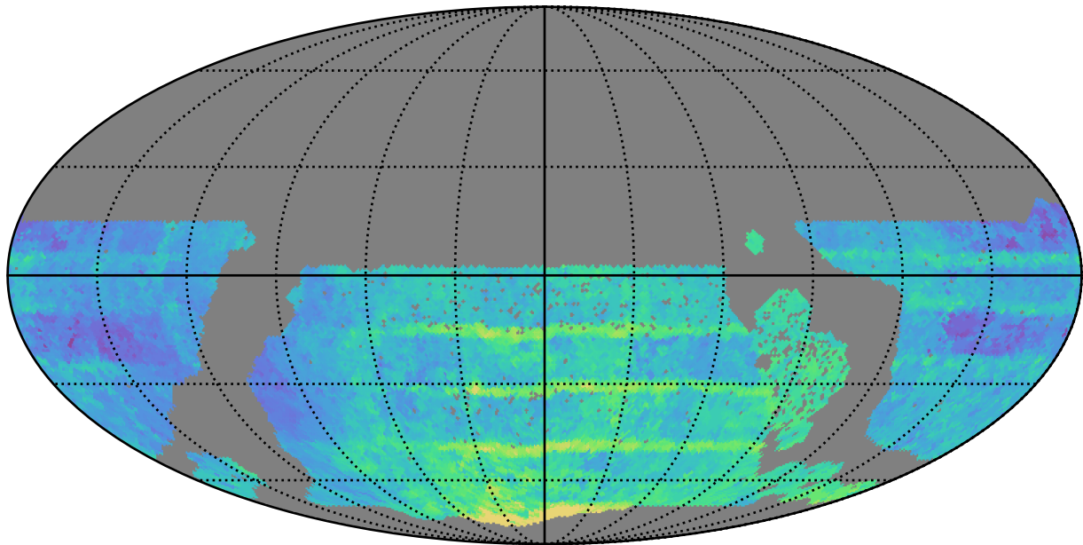
ddf_acor_sf20_lsf30_lsr10_v3.4_10yrs WFD all bands: Median Season Length
