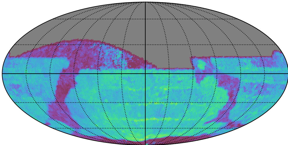
ddf_acor_sf20_lsf30_lsr10_v3.4_10yrs All sky z band: Median Season Length
