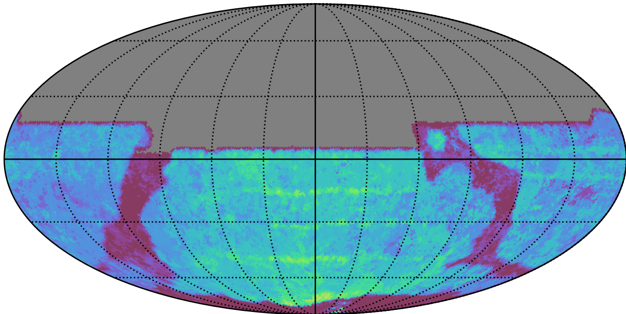
ddf_acor_sf20_lsf30_lsr10_v3.4_10yrs All sky y band: Median Season Length
