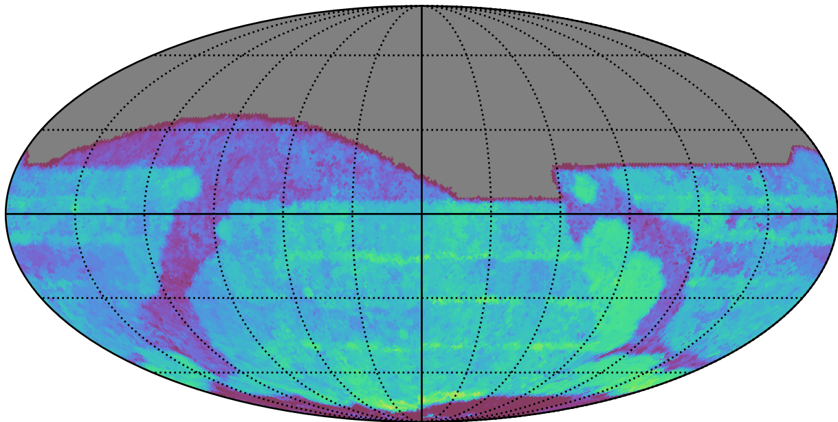
ddf_acor_sf20_lsf30_lsr10_v3.4_10yrs All sky r band: Median Season Length
