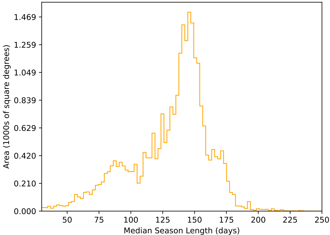
ddf_acor_sf20_lsf30_lsr10_v3.4_10yrs All sky r band: Median Season Length
