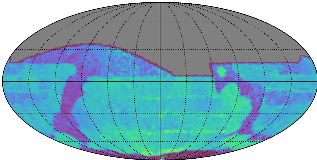
ddf_acor_sf20_lsf30_lsr10_v3.4_10yrs All sky i band: Median Season Length
