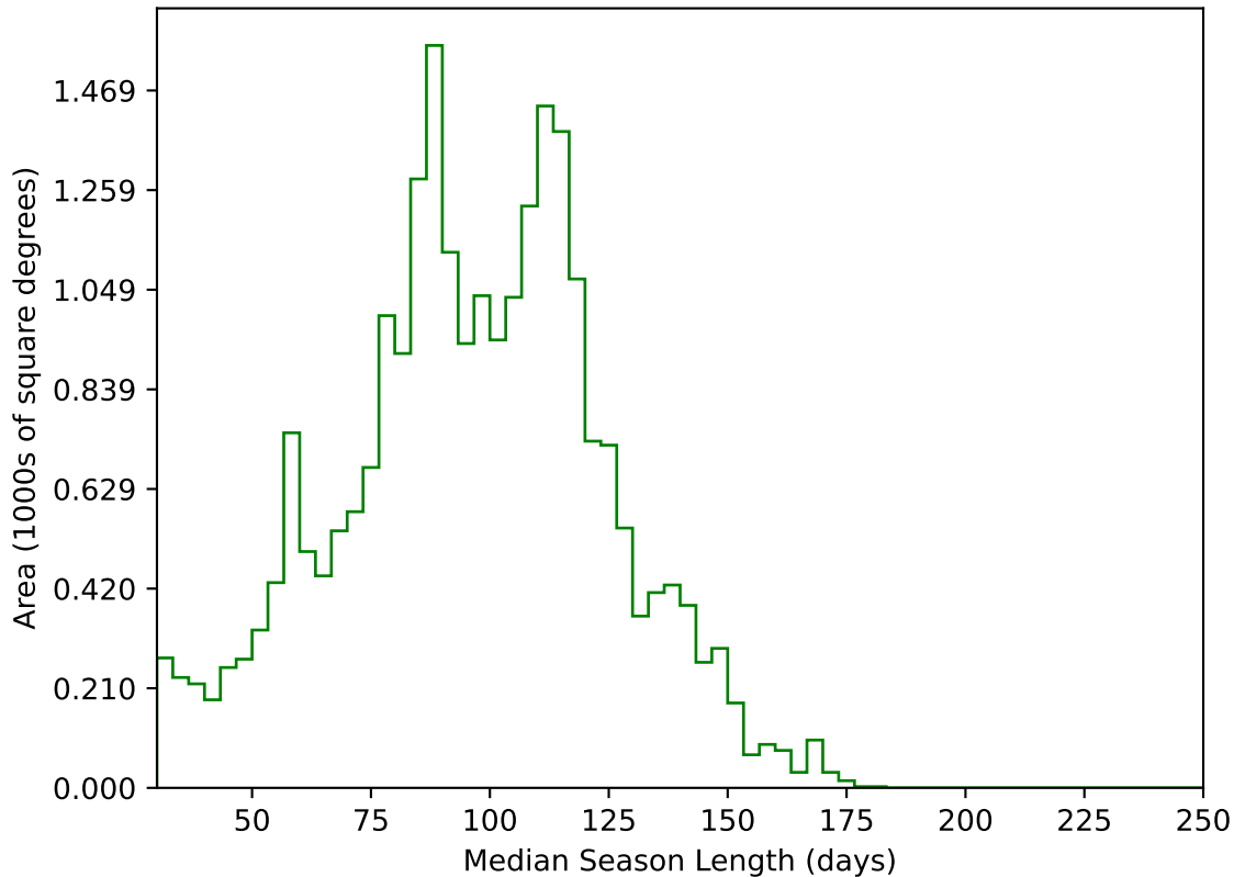
ddf_acor_sf20_lsf30_lsr10_v3.4_10yrs All sky g band: Median Season Length
