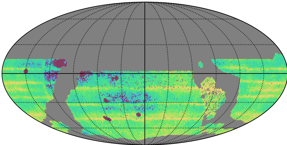
ddf_acor_sf20_lsf30_lsr10_v3.4_10yrs WFD: Median Intra-Night Gap
