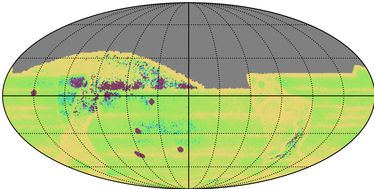
ddf_acor_sf20_lsf30_lsr10_v3.4_10yrs All sky: Median Intra-Night Gap
