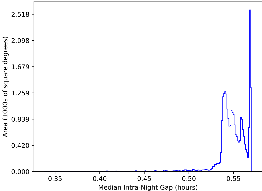
ddf_acor_sf20_lsf30_lsr10_v3.4_10yrs All sky: Median Intra-Night Gap
