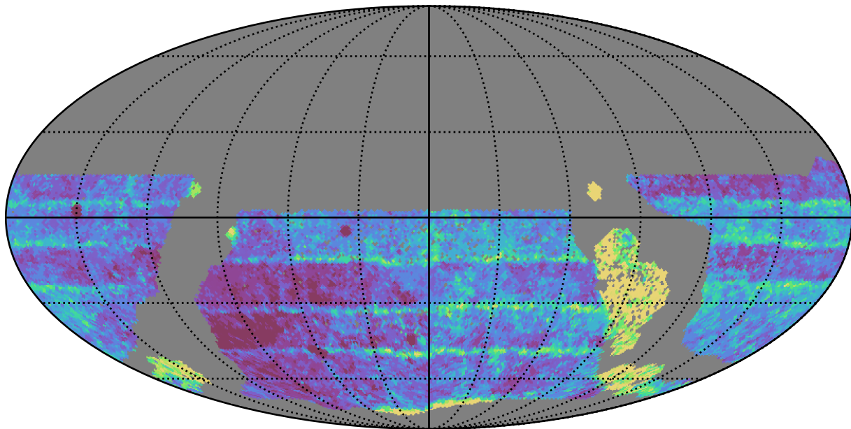
ddf_acor_sf20_lsf30_lsr10_v3.4_10yrs WFD z band: Median Inter-Night Gap
