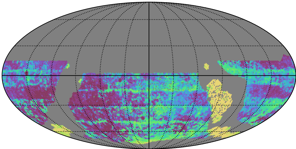
ddf_acor_sf20_lsf30_lsr10_v3.4_10yrs WFD y band: Median Inter-Night Gap
