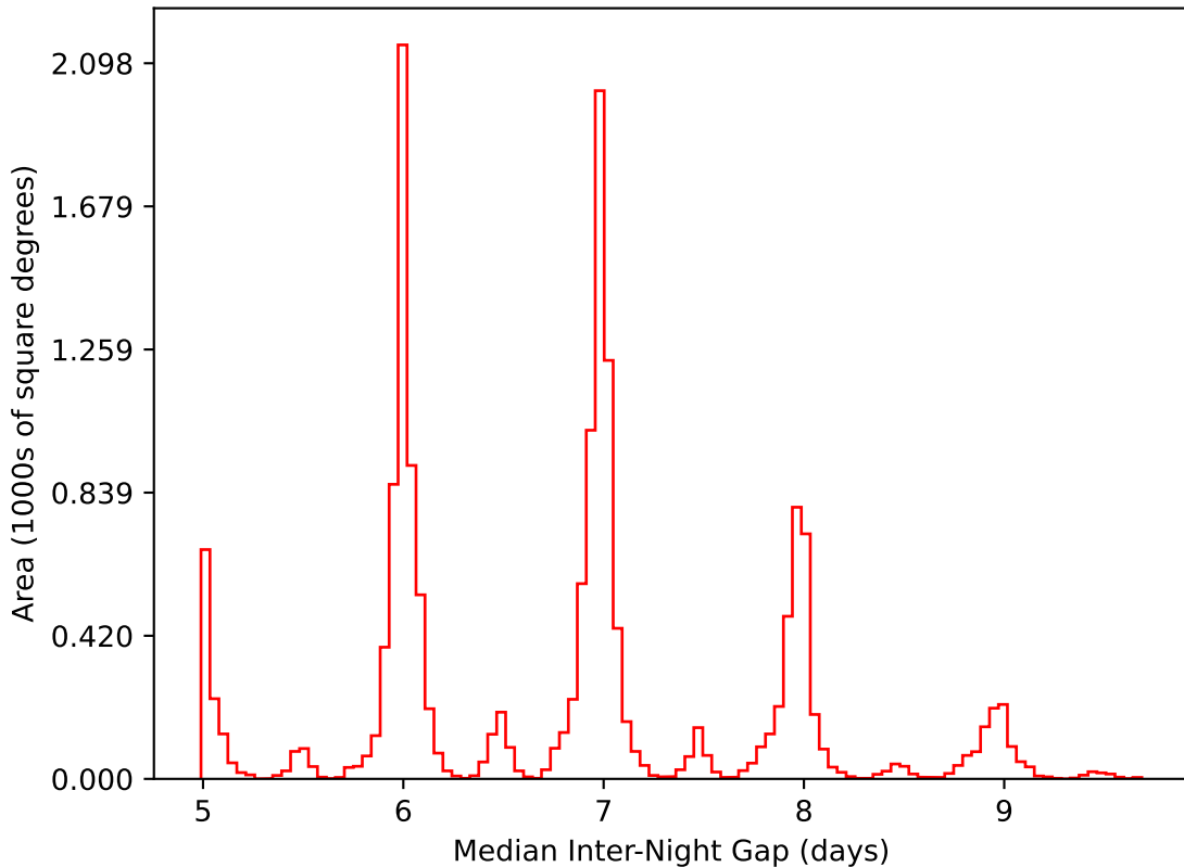
ddf_acor_sf20_lsf30_lsr10_v3.4_10yrs WFD i band: Median Inter-Night Gap
