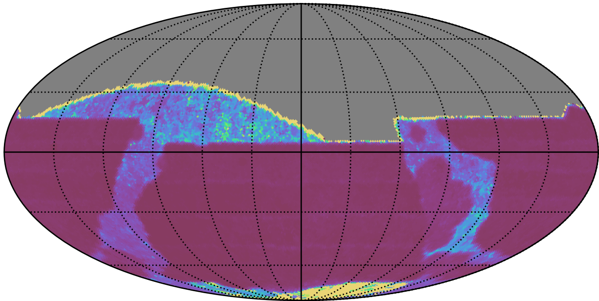
ddf_acor_sf20_lsf30_lsr10_v3.4_10yrs All sky z band: Median Inter-Night Gap
