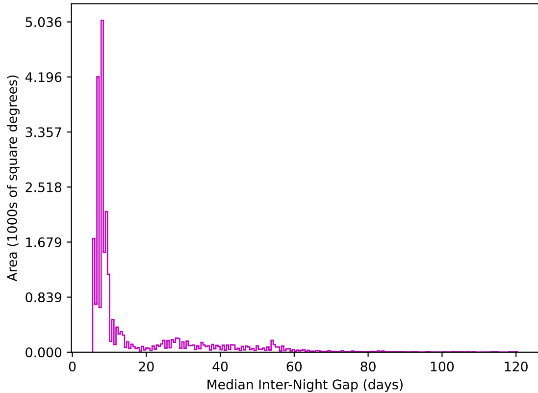
ddf_acor_sf20_lsf30_lsr10_v3.4_10yrs All sky z band: Median Inter-Night Gap
