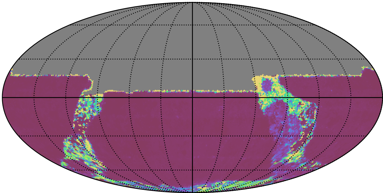
ddf_acor_sf20_lsf30_lsr10_v3.4_10yrs All sky u band: Median Inter-Night Gap
