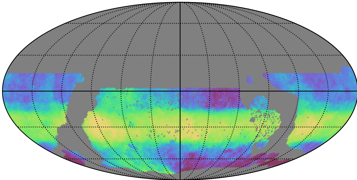
ddf_acor_sf20_lsf30_lsr10_v3.4_10yrs WFD z band: Median HA
