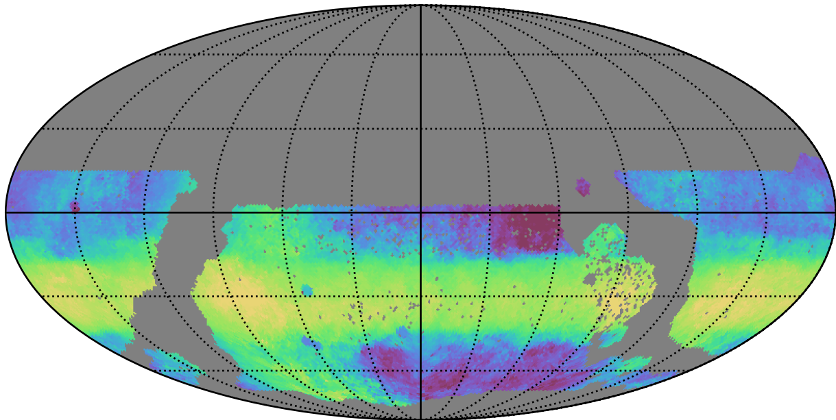
ddf_acor_sf20_lsf30_lsr10_v3.4_10yrs WFD y band: Median HA
