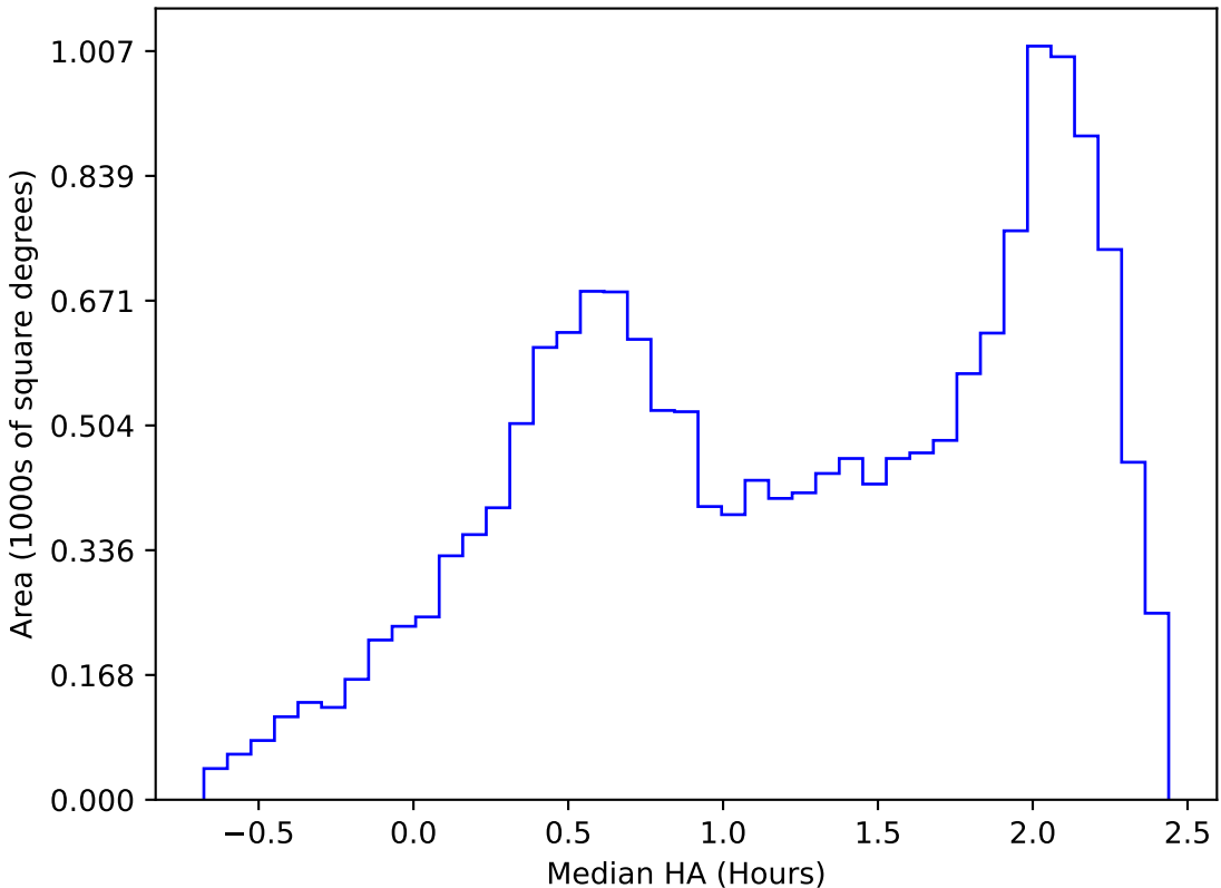
ddf_acor_sf20_lsf30_lsr10_v3.4_10yrs WFD y band: Median HA
