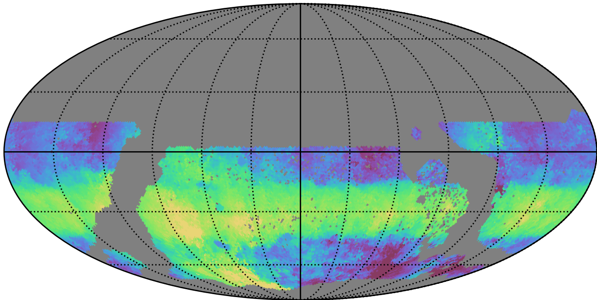
ddf_acor_sf20_lsf30_lsr10_v3.4_10yrs WFD u band: Median HA
