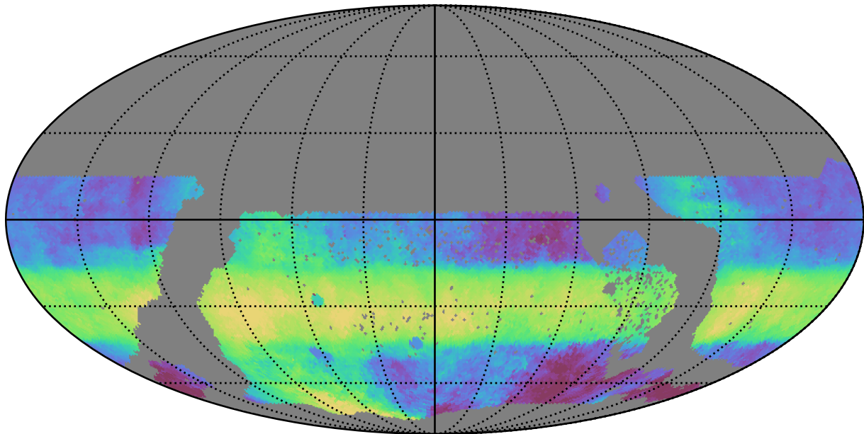
ddf_acor_sf20_lsf30_lsr10_v3.4_10yrs WFD r band: Median HA
