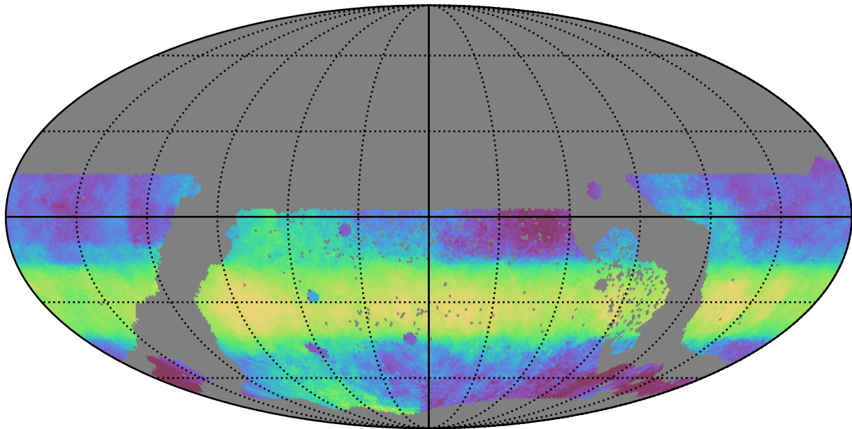
ddf_acor_sf20_lsf30_lsr10_v3.4_10yrs WFD i band: Median HA
