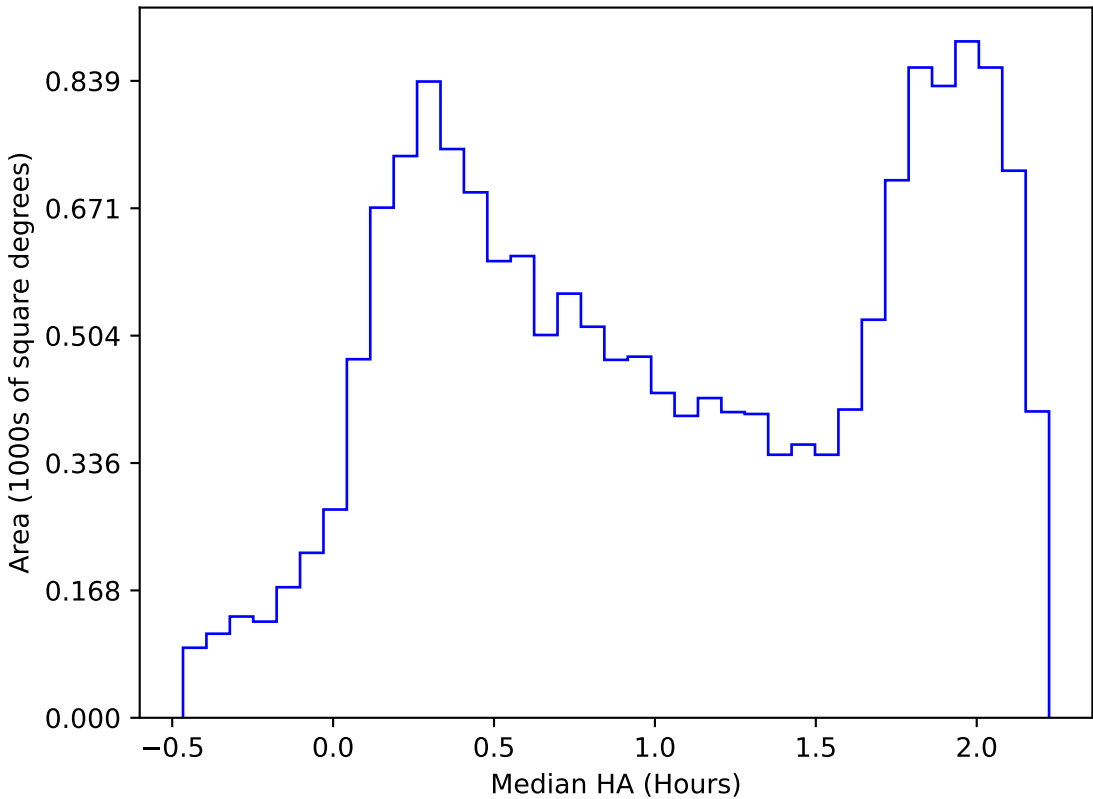
ddf_acor_sf20_lsf30_lsr10_v3.4_10yrs WFD i band: Median HA
