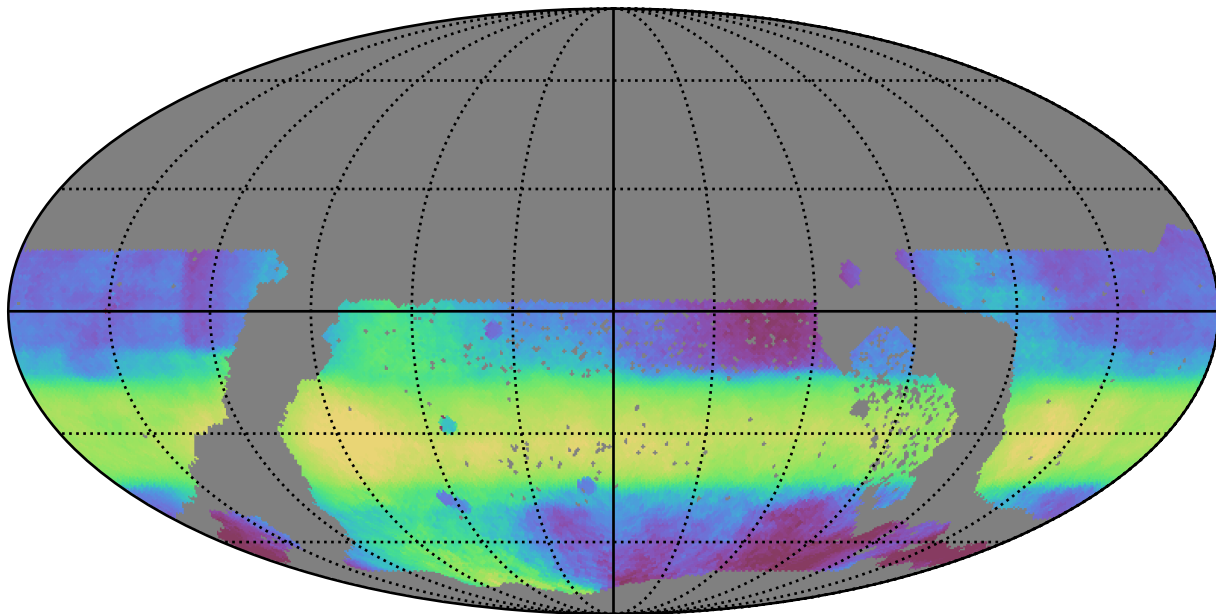
ddf_acor_sf20_lsf30_lsr10_v3.4_10yrs WFD all bands: Median HA
