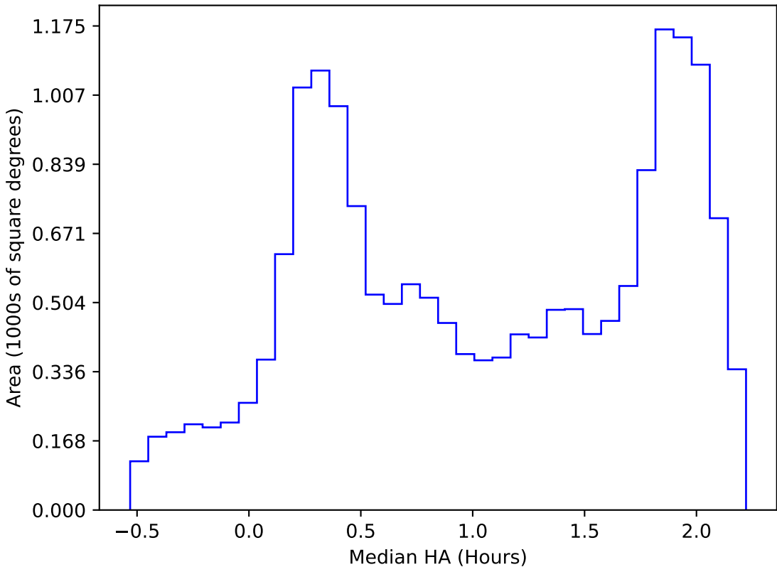
ddf_acor_sf20_lsf30_lsr10_v3.4_10yrs WFD all bands: Median HA
