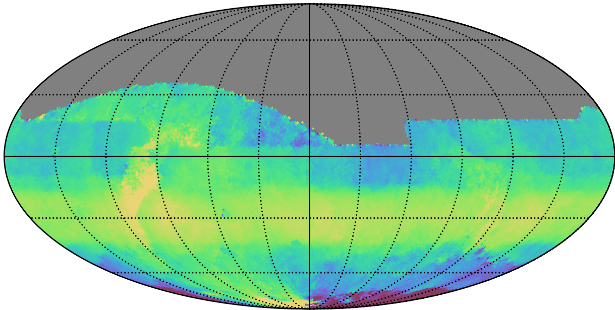
ddf_acor_sf20_lsf30_lsr10_v3.4_10yrs All sky z band: Median HA
