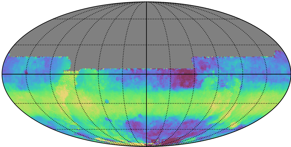
ddf_acor_sf20_lsf30_lsr10_v3.4_10yrs All sky y band: Median HA
