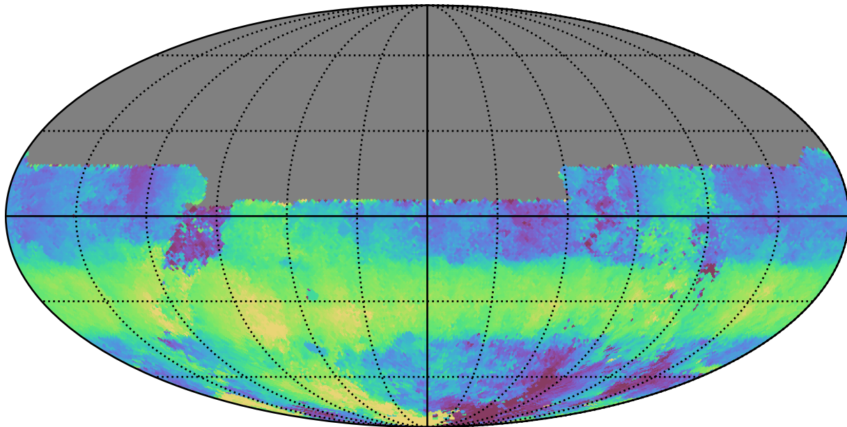
ddf_acor_sf20_lsf30_lsr10_v3.4_10yrs All sky u band: Median HA
