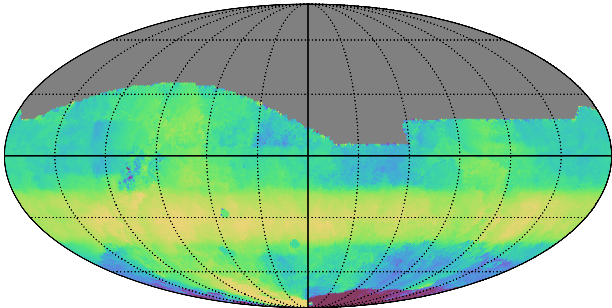
ddf_acor_sf20_lsf30_lsr10_v3.4_10yrs All sky r band: Median HA
