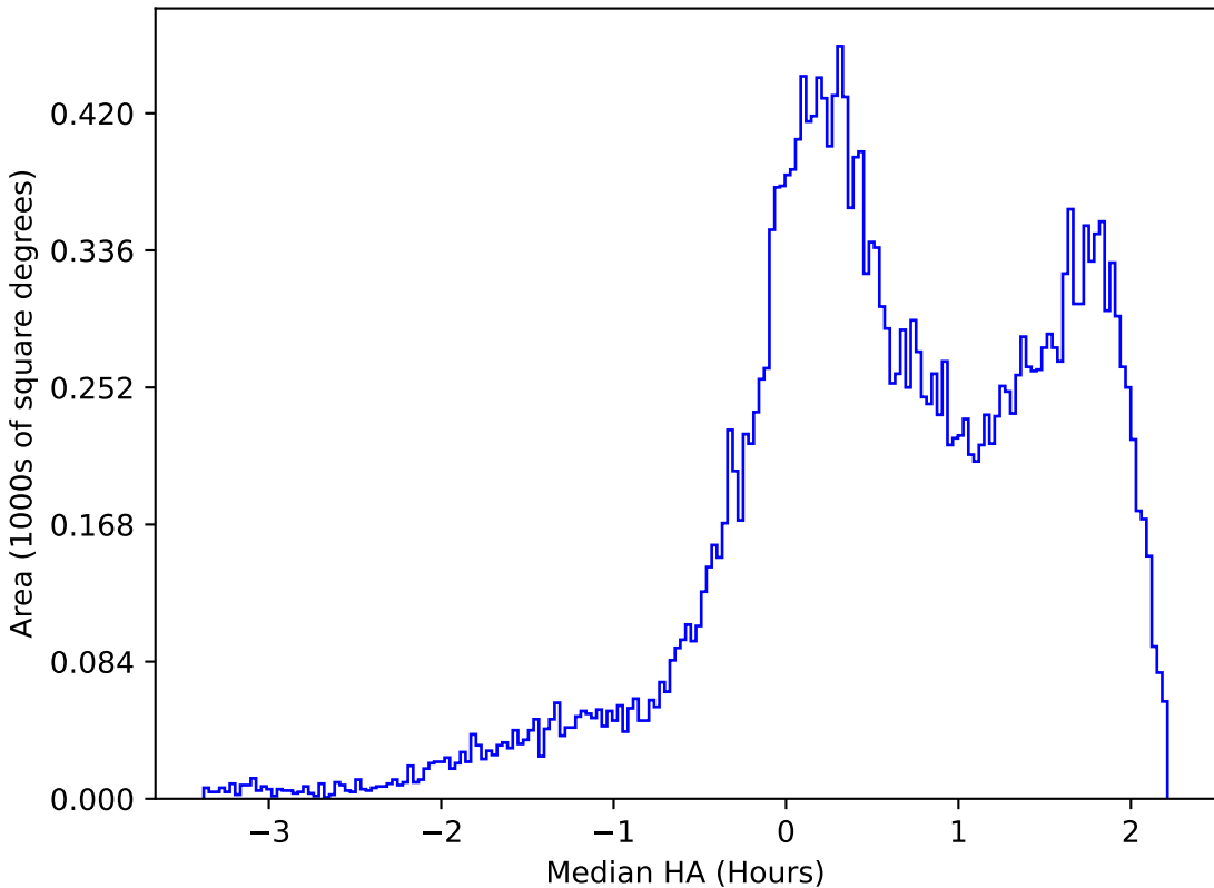
ddf_acor_sf20_lsf30_lsr10_v3.4_10yrs All sky g band: Median HA
