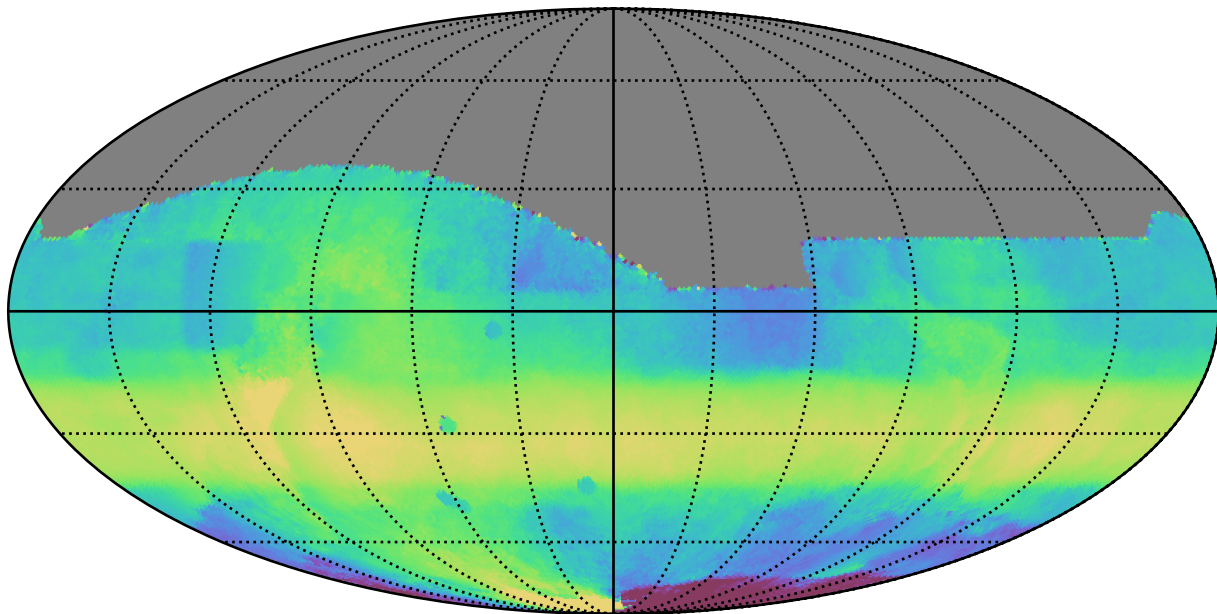
ddf_acor_sf20_lsf30_lsr10_v3.4_10yrs All sky all bands: Median HA
