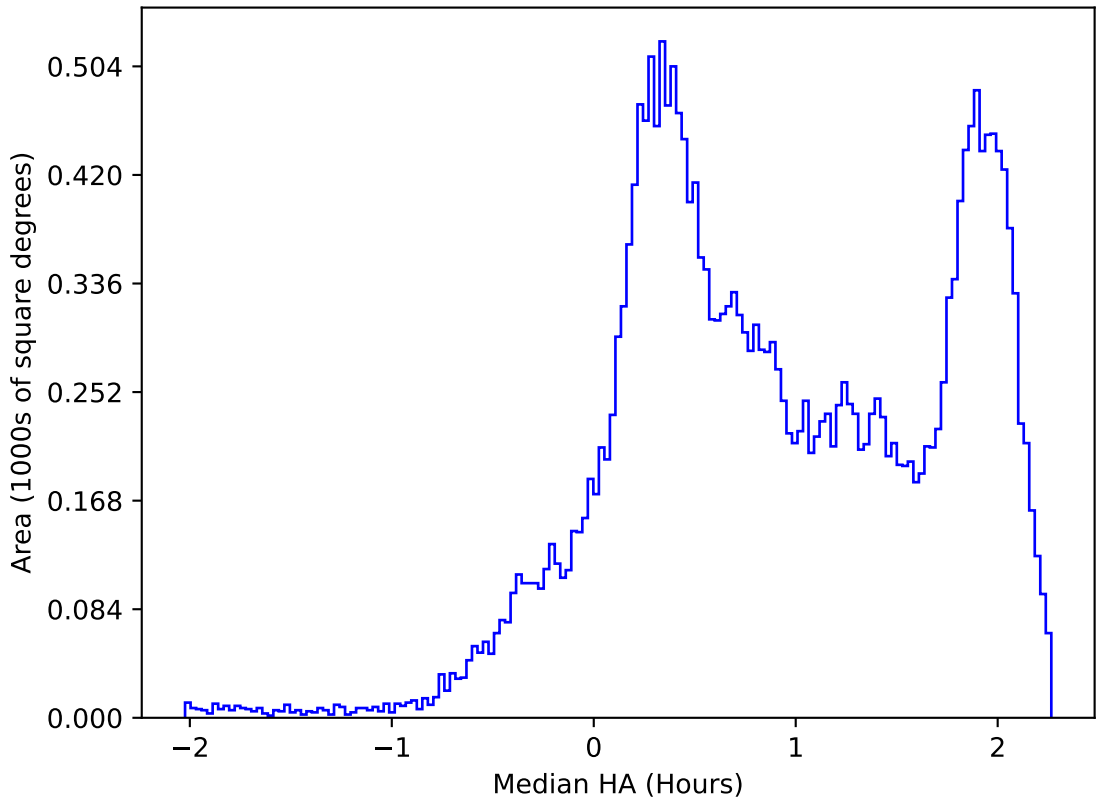
ddf_acor_sf20_lsf30_lsr10_v3.4_10yrs All sky all bands: Median HA
